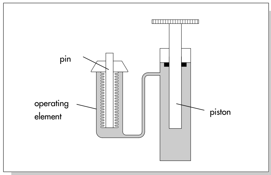
Fig. 7: Set point adjustment at temperature sensor
