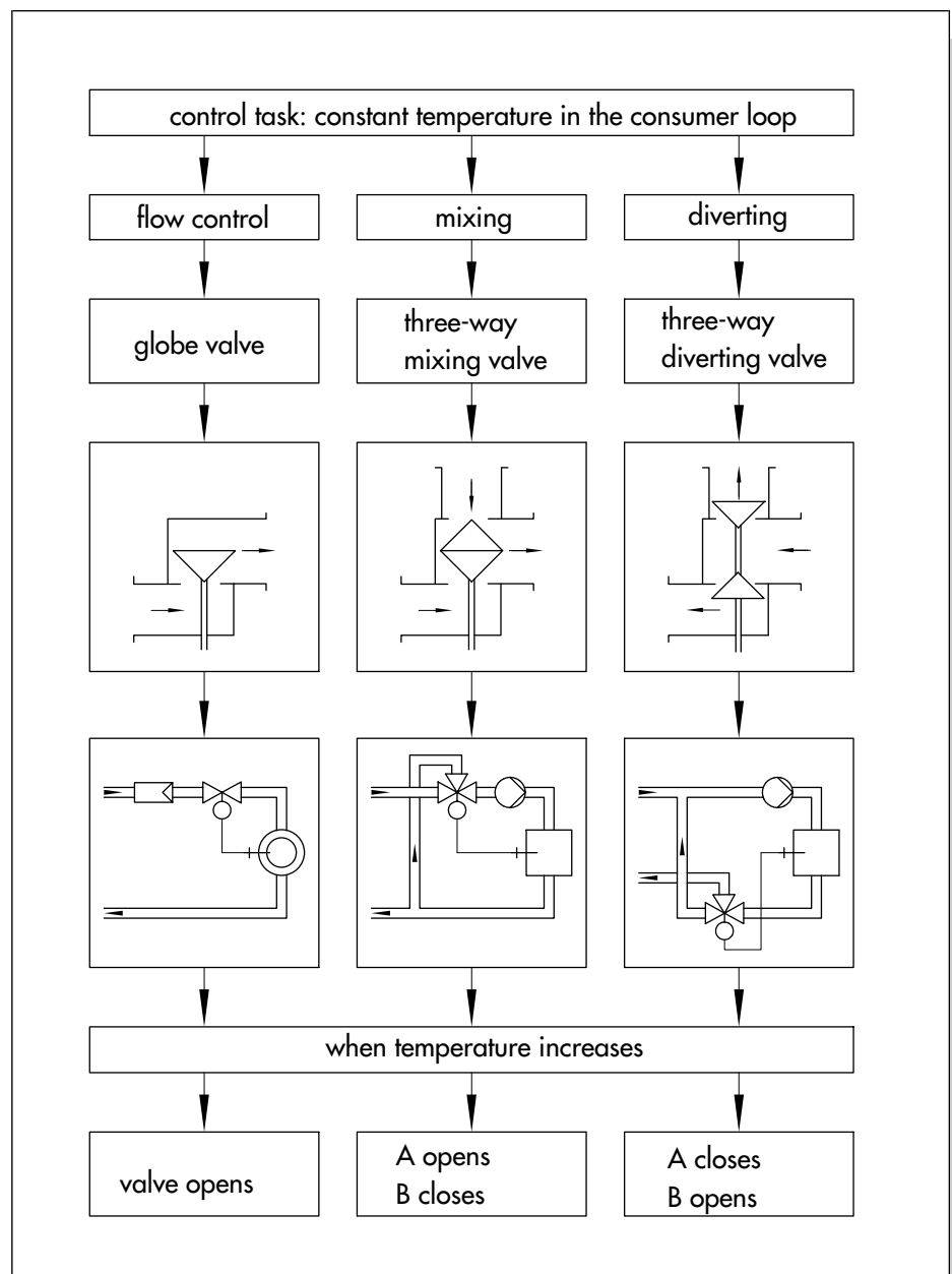
Fig. 15: Example of a cooling system
