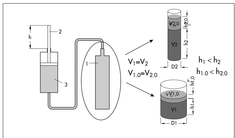
Fig. 2: Expansion of a liquid in a cylinder
