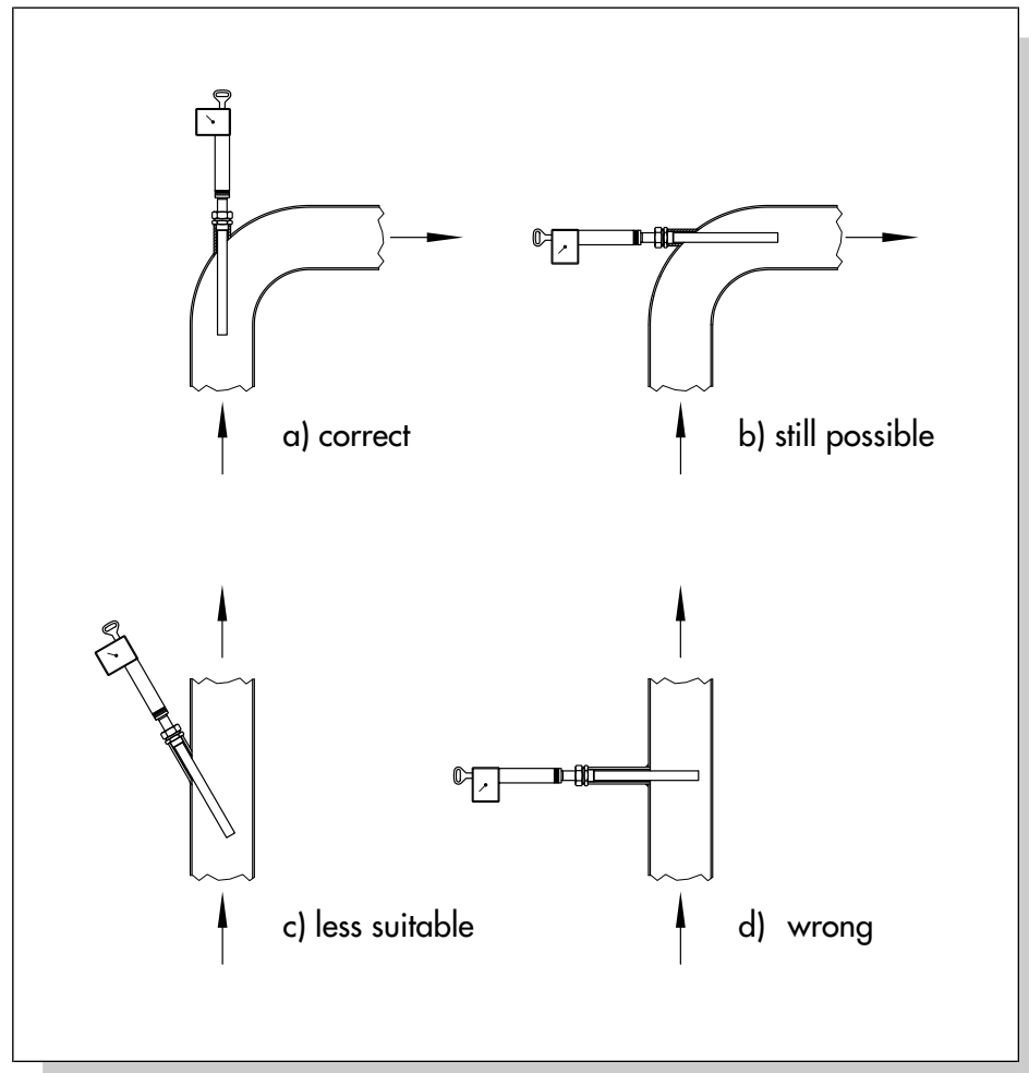
Fig. 9: Sensor locations
